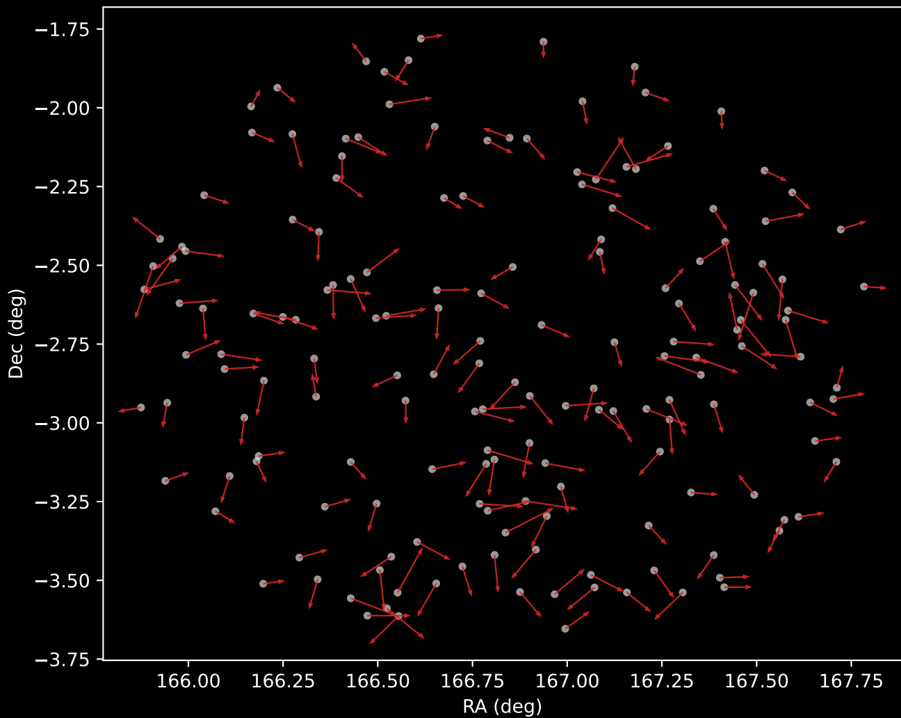
GALAH DR4 Cluster 6 Proper Motion Vectors (n=167)
