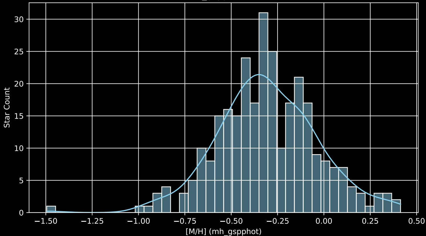
GALAH DR4 Field: [722] [M/H] (mh_gspphot) (n= 291)
