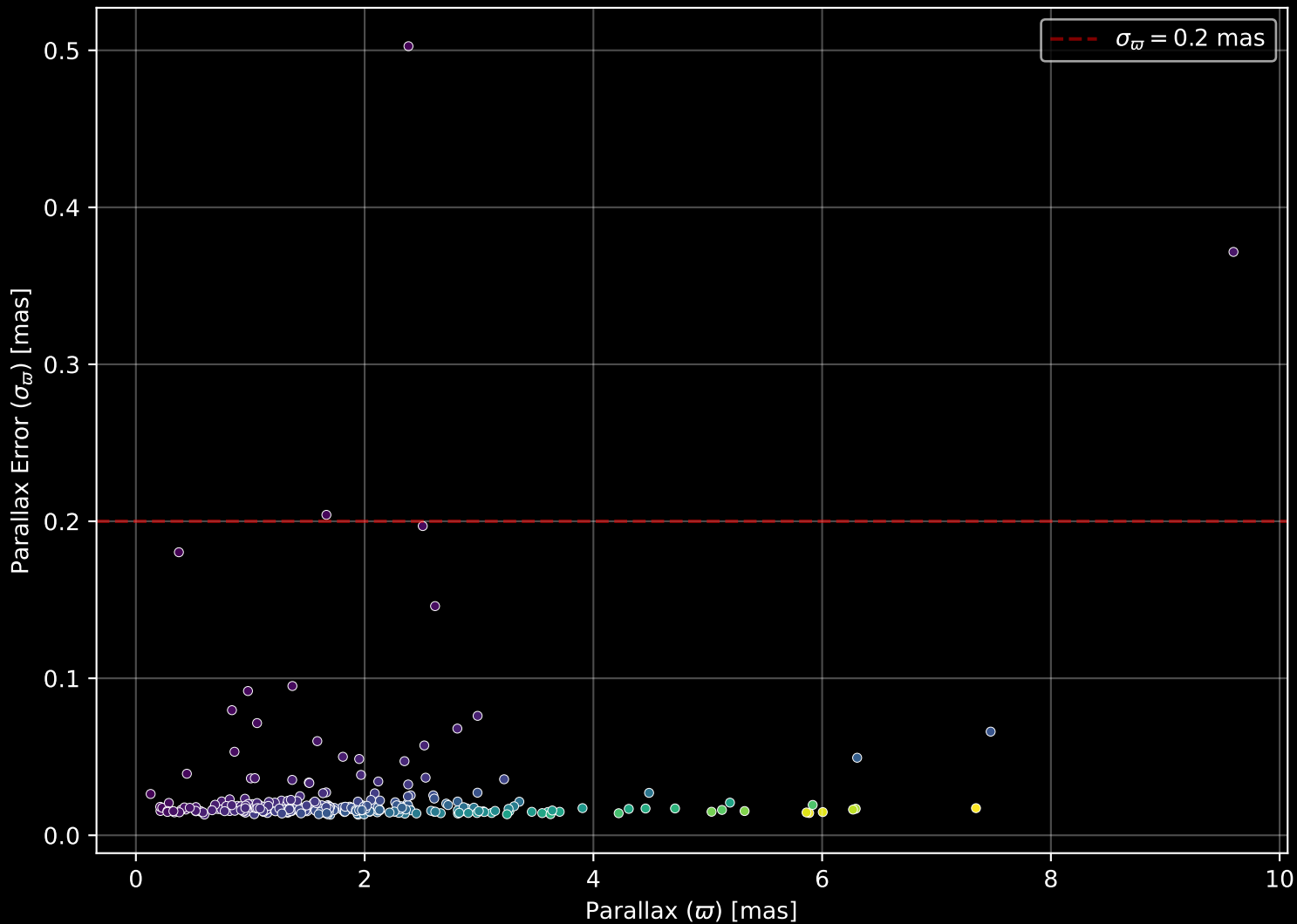
GALAH DR4 Field: [722] Parallax Quality (n= 291)
