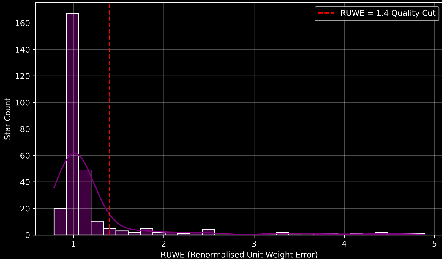
GALAH DR4 Field [722] RUWE Distribution (n= 283)
