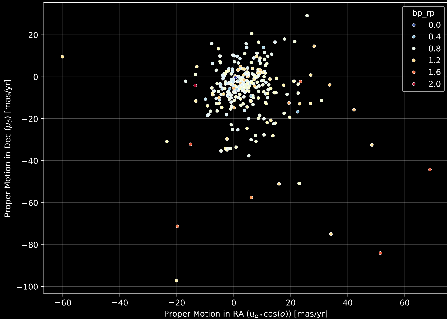
GALAH DR4 Field: [722] Proper Motion Diagram (n= 291)
