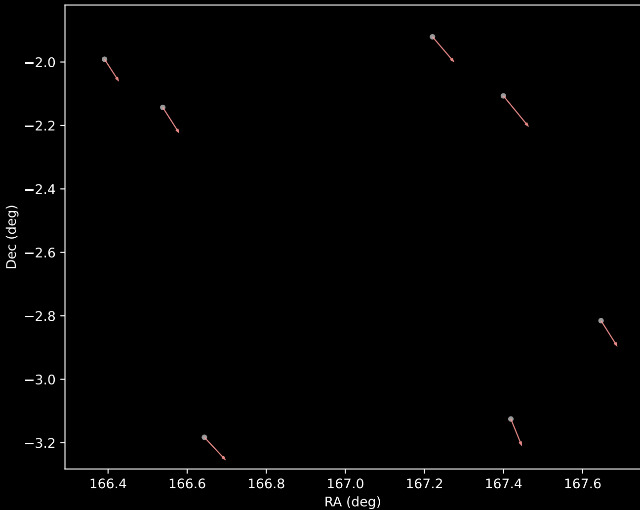
GALAH DR4 Cluster 7 Proper Motion Vectors (n=7)
