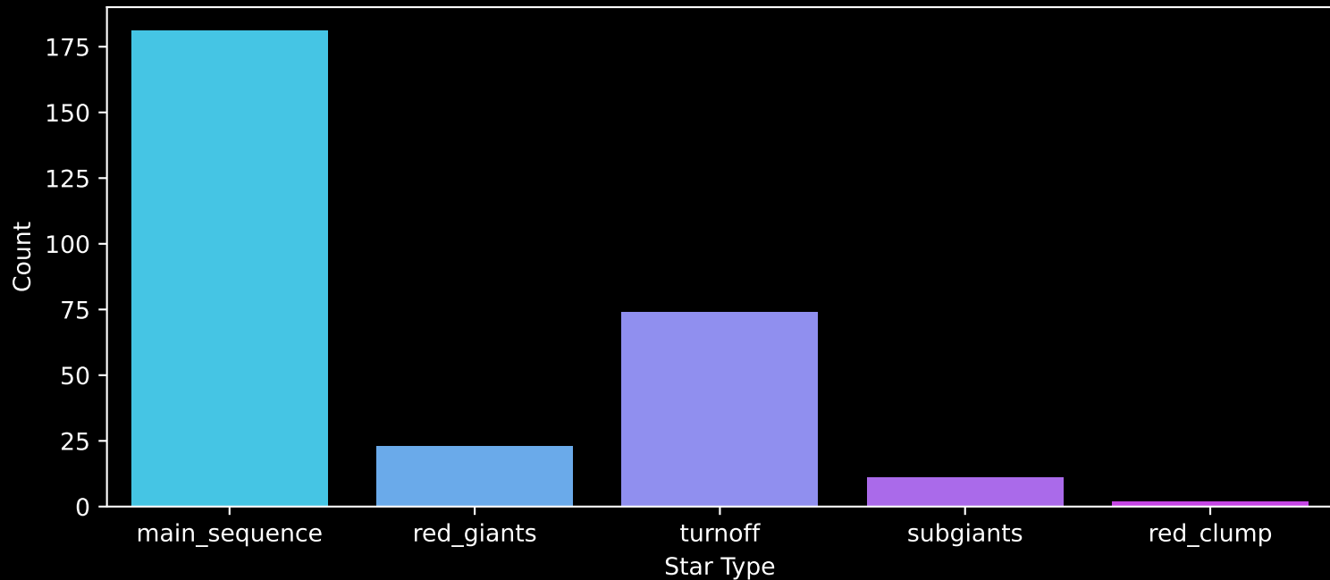
GALAH DR4 Field: [722] Count plot of Star Type
